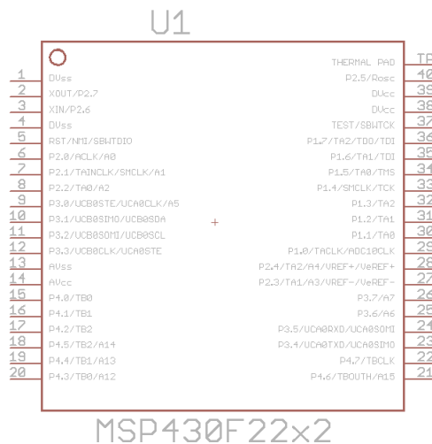
Figure 6.1: MSP430F2274 Schematic
